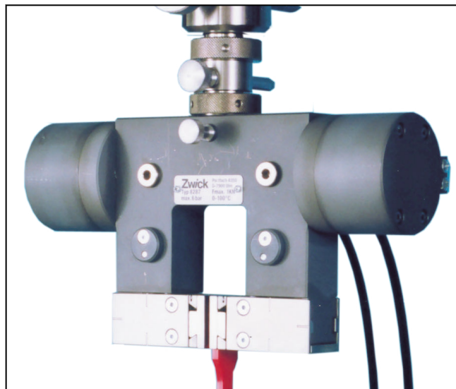
Pneumatic grips, Type 8287, Fmax 1 kN: detail
